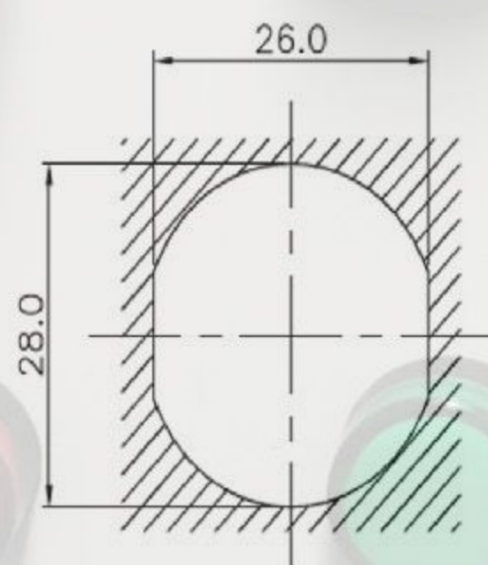
Panel Cutout
